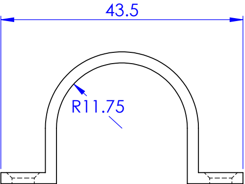
Bracket UA49346
