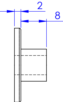
Feeder Cap UA49340
