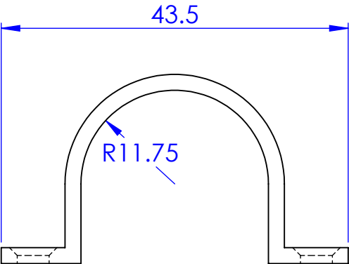
Bracket UA49346
