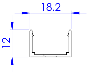
Housing UA49248
