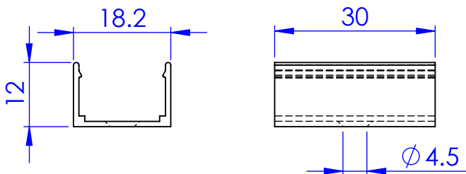
Bracket UA49249
