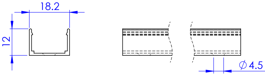
Housing UA49248
