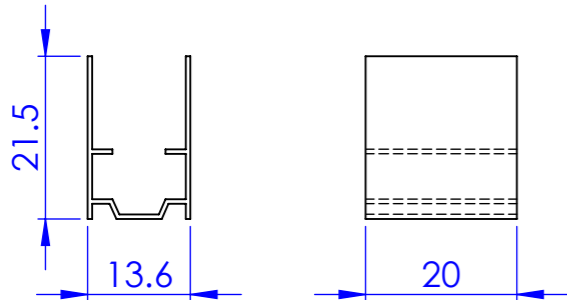
Bracket UA49246
