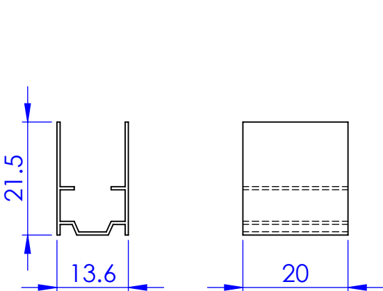
Bracket UA49246
