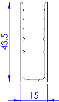
Housing UA49245
