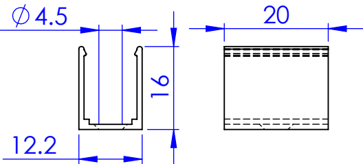
Bracket UA49237
