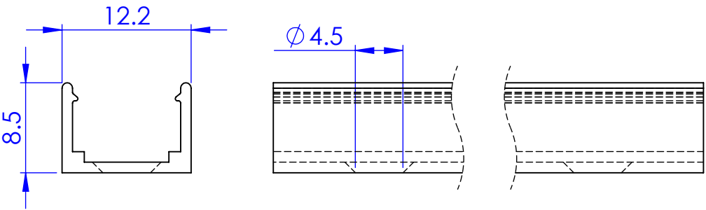
Housing UA49436
