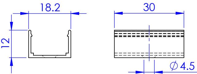
Bracket UA49219
