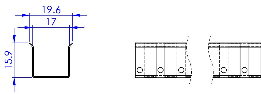
Bendable Housing UA49220
