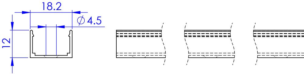
Housing UA49218
