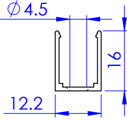
Housing UA49236
