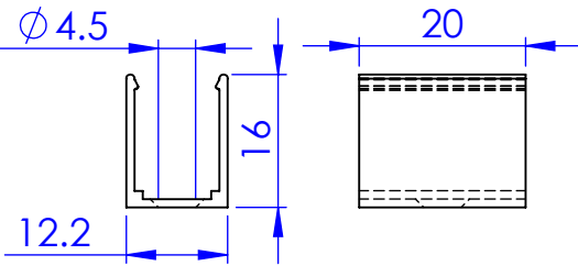
Bracket UA49237
