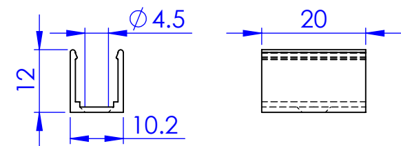
Bracket UA49231
