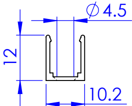
Housing UA49230
