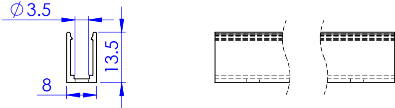
Housing UA49224
