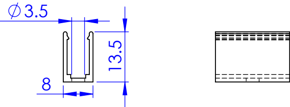
Bracket UA49225
